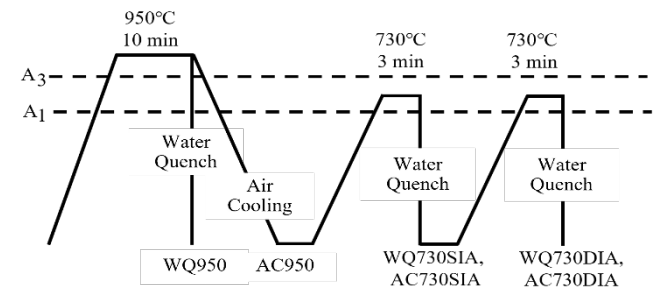
Figure 2. Heat treatment profile used in this study.
